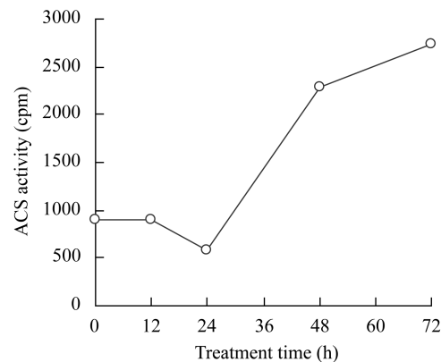
Fig. 4 Assay of ACS activity
