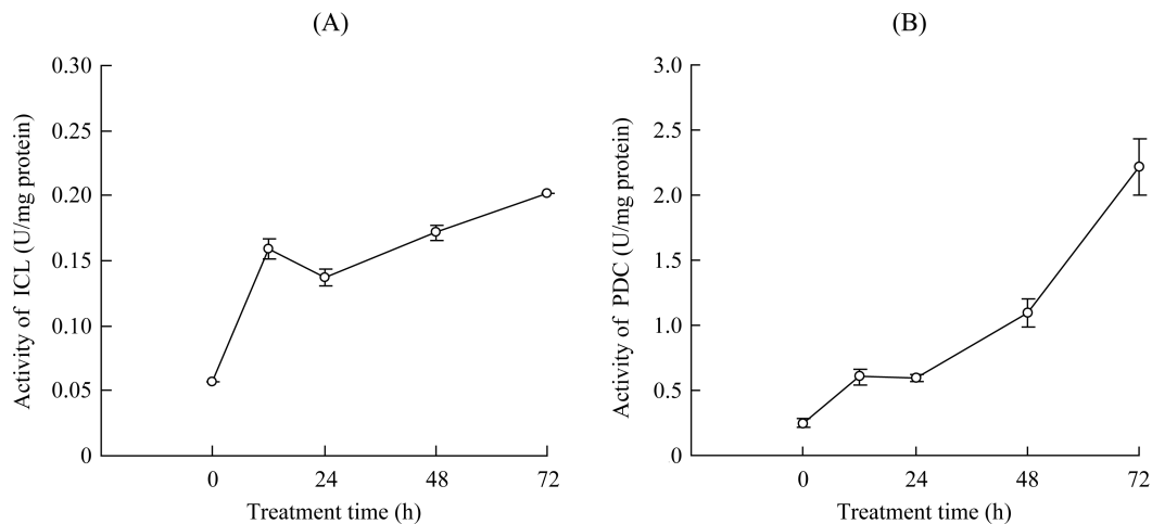
Fig. 3 Activity assays of ICL and PDC
